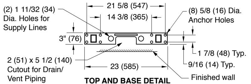
TOP AND BASE DETAIL
