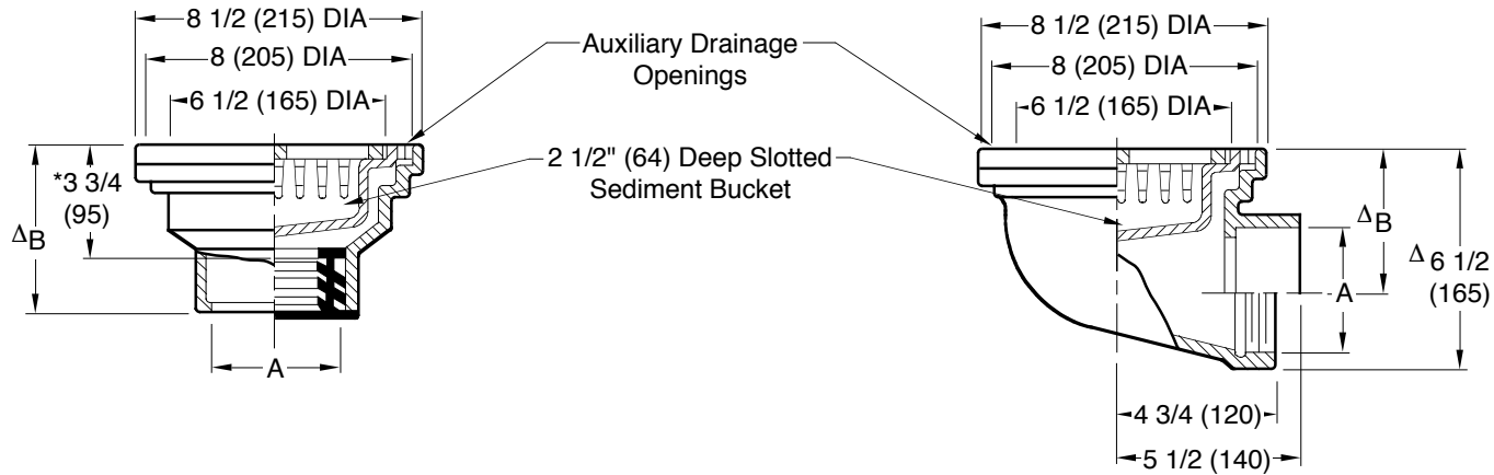
Fig. 2210C. . . . CAULK OUTLET Fig. 2210Y. . . . NO-HUB OUTLET
